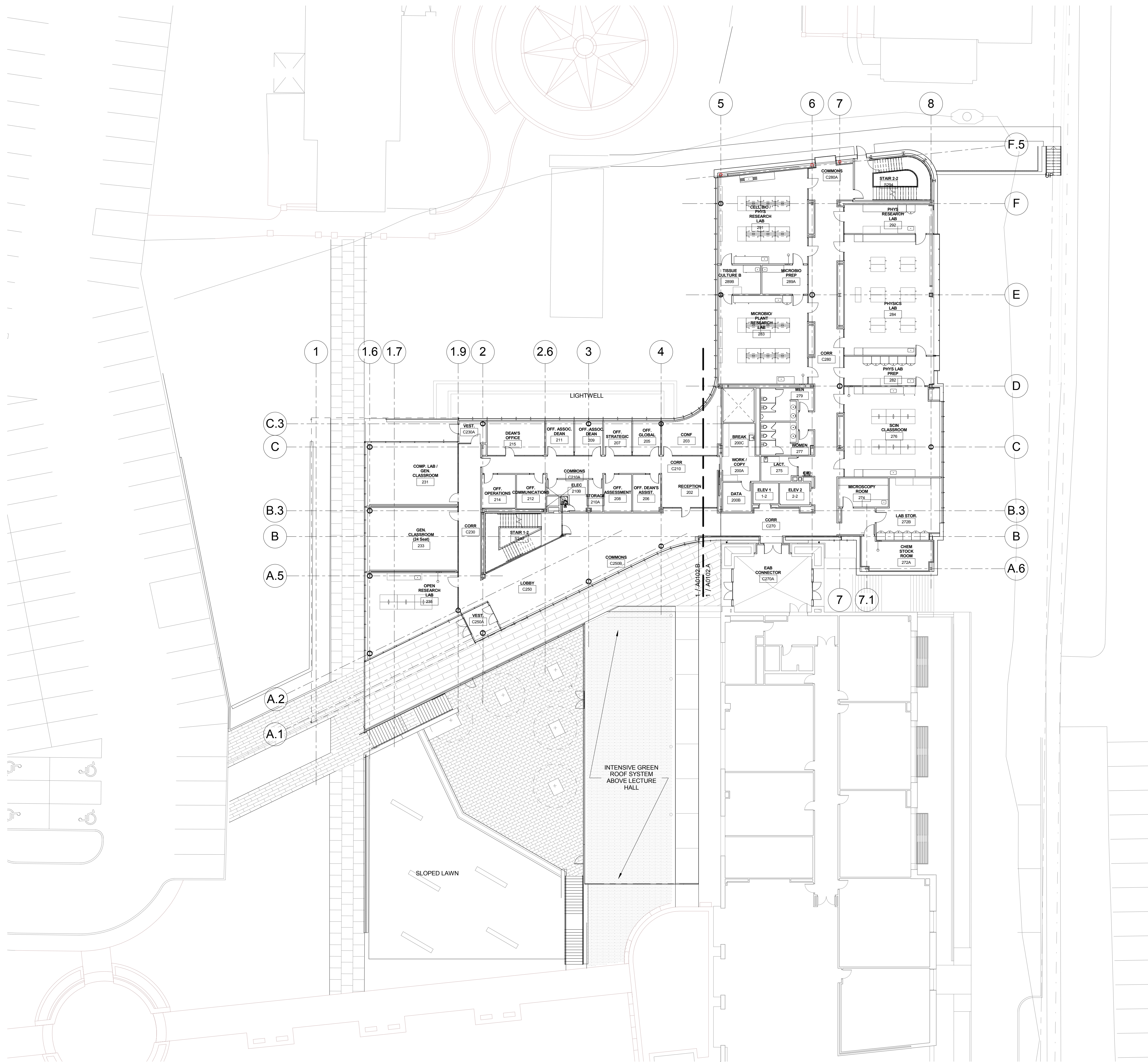
1 LEVEL 02 1/16" = 1'-0"
